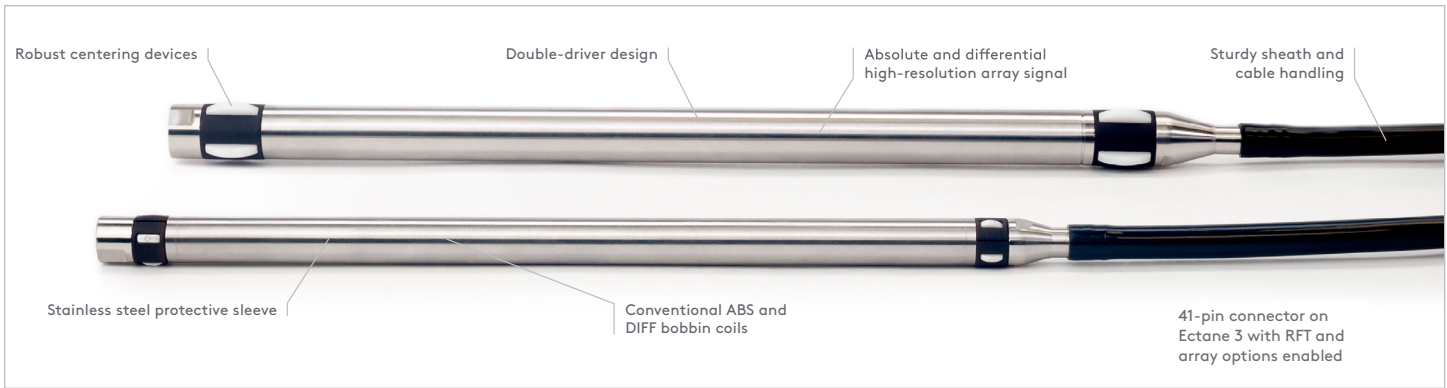
Figure 1: Annotated breakdown of the RFA probe.
